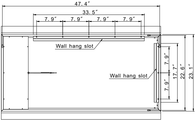
REAR VIEW
