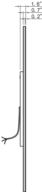
RIGHT SIDE
