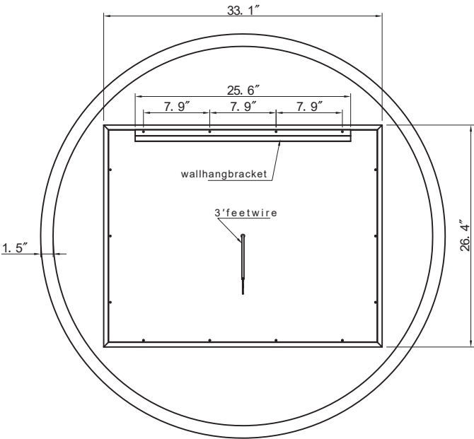
REAR VIEW
