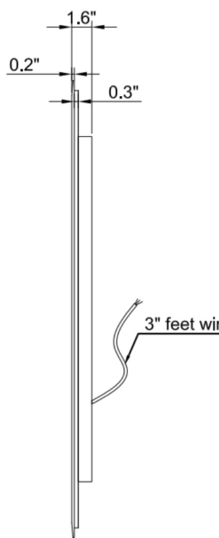
LEFT VIEW
