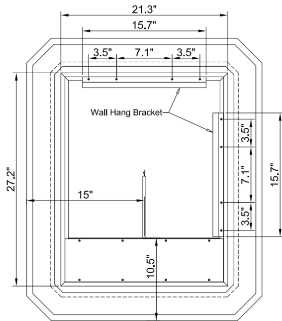
REAR VIEW
