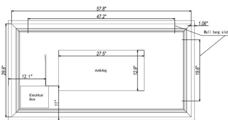
REAR VIEW
