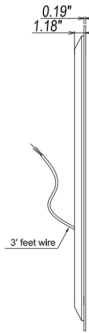
LEFT VIEW
