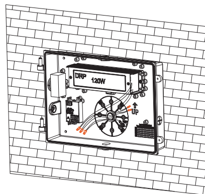
Step 6: Wiring
