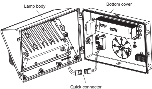
Step 2: Unplug the quick connector and separate the lamp body from the bottom cover
