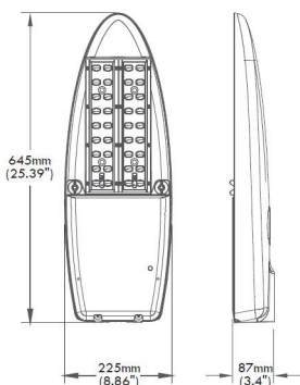
SGC80/SGD120 (Type 2)
