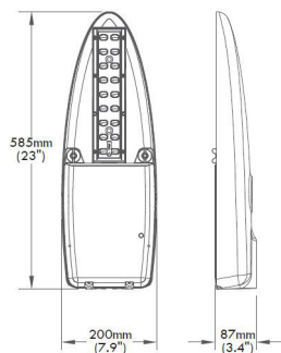
SGB30/SGC40/SGD60/SGE80 (Type 1)
