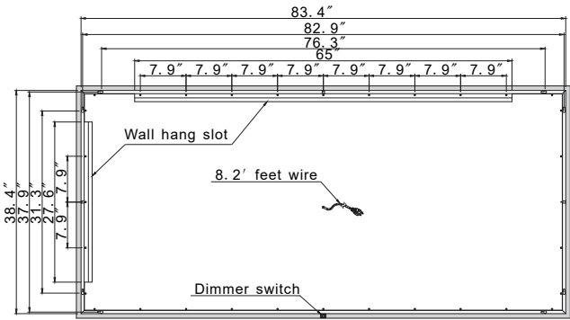
REAR VIEW
