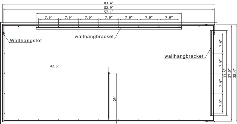
REAR VIEW
