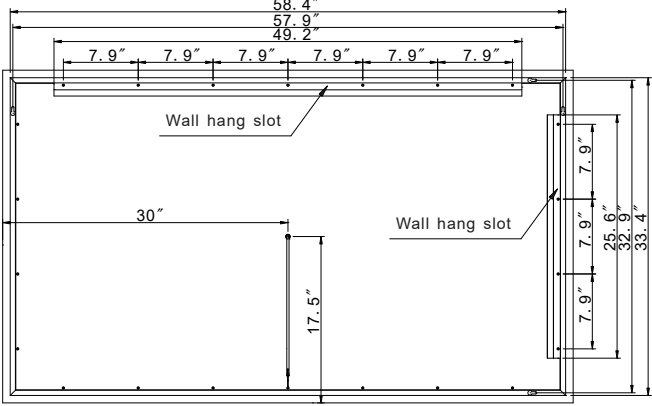
REAR VIEW
