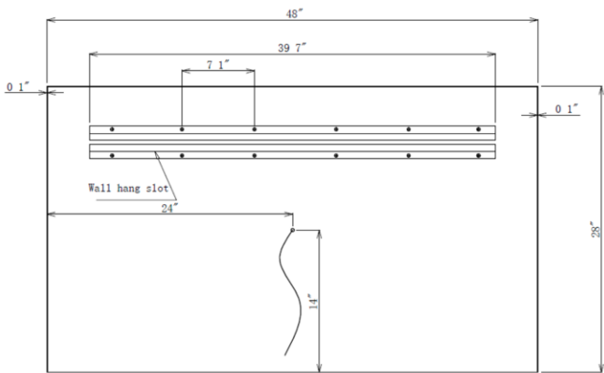
REAR VIEW
